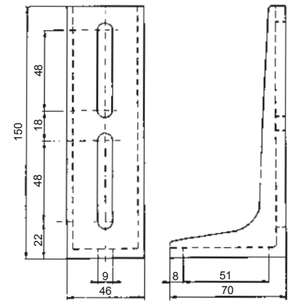
support bracket 03
