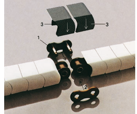
Connecting link
